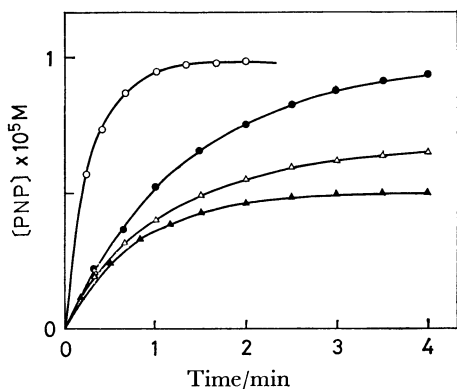
Fig. 3. The time course of the p -nitrophenol (PNP) release from C 2 -BNPP by several hydroxamates in the presence of the CTAB micelle. 30 °C, pH 8.8, 0.02 M borate buffer, \mu=0.01 (KCl), [CTAB]= 1.00 \times 10^{-3} M, [hydroxamate]= 5.00 \times 10^{-5} M, [C 2 -BNPP]= 5.00 \times 10^{-6} M. p -Nitrophenolate anion: \lambda_{\max} 400 nm, \epsilon=1.81 \times 10^4 . C 18 -MHA: —○—, C 18 -HA: —●—, C 18 -PHA: —△—, C 12 N + -C 2 -MHA: —▲—.
