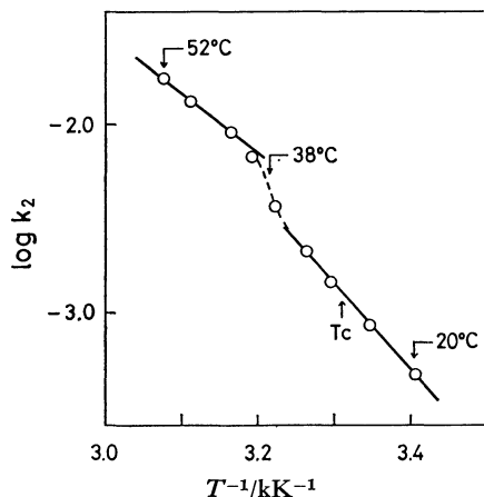
Fig. 6. Arrhenius plots for k_{2, \text{obsd}} for the reaction of \text{C}_{18}\text{-BNPP} with \text{C}_{18}\text{-MHA} in the 2\text{C}_{16}\text{N}+2\text{C}_1 membrane.
