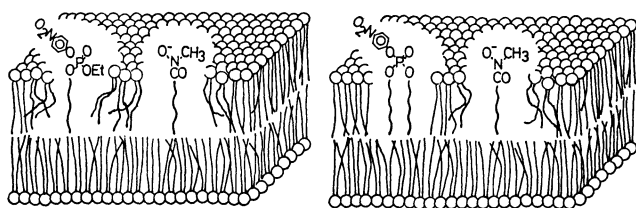
Fig. 7. Schematic illustration of nucleophiles and substrates in the membrane matrix.
